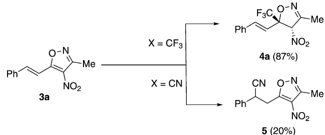
Scheme 3. Addition of trimethylsilyl carbon nucleophiles to 3-methyl-4-nitro-5-styrylisoxazole 3a . Reaction conditions: \text{Me}_3\text{SiX} (2.0 equiv), NaOAc (1.5 equiv), [\text{CH}_3(\text{CH}_2)_{15}\text{N}(\text{CH}_3)_3]\text{Br} (30 mol %), DMF, RT; 1 M HCl aq.
